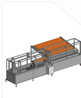
Fully Automatic Paper Core Cutting Machine With Auto Loading and Auto Unliading
