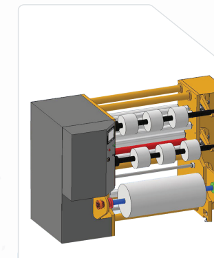
Duplex System Slitter Rewinder Machine
